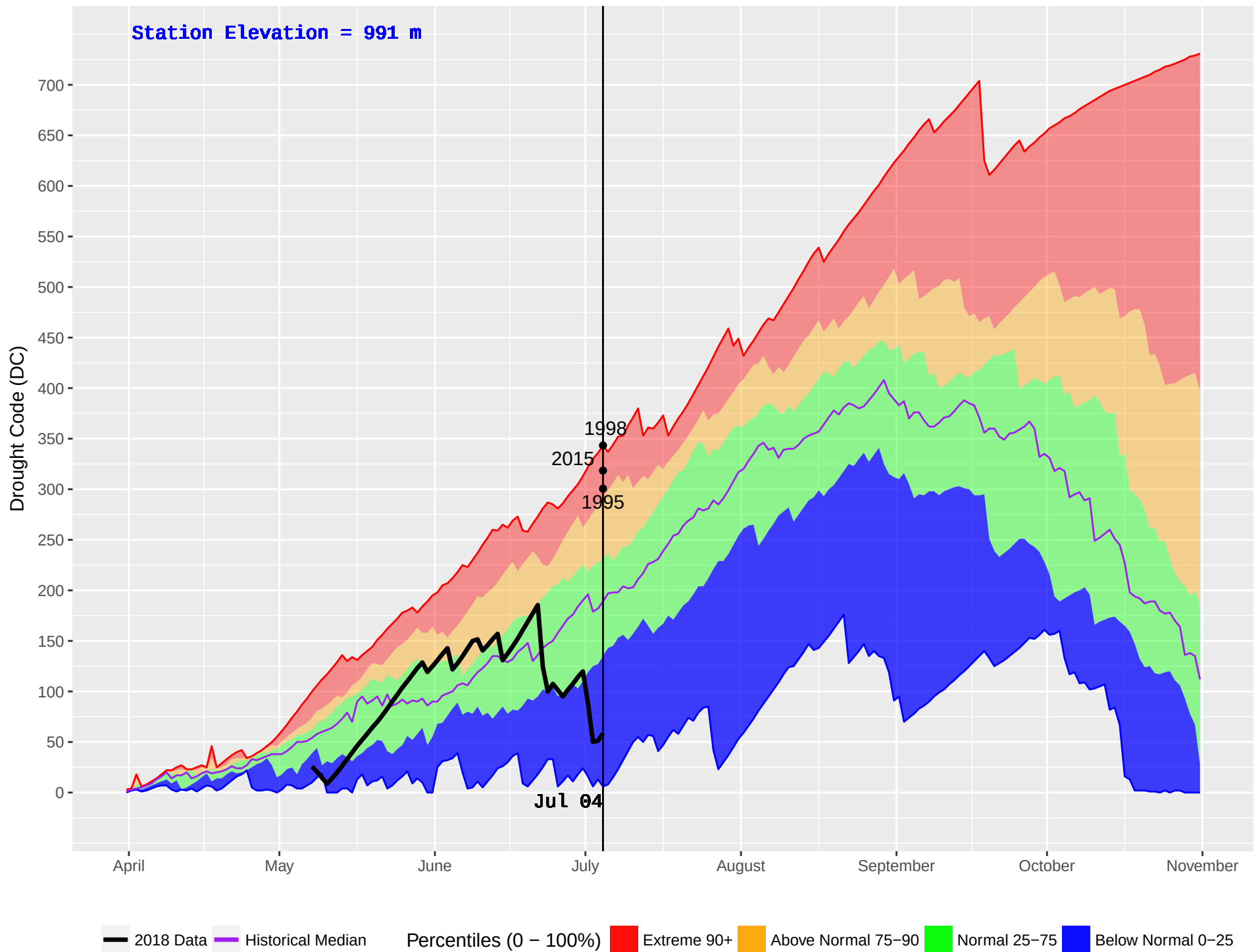
TROUT LAKE (387) : Historical (1987–2016) and Current (2018) Noon Drought Code (DC)
