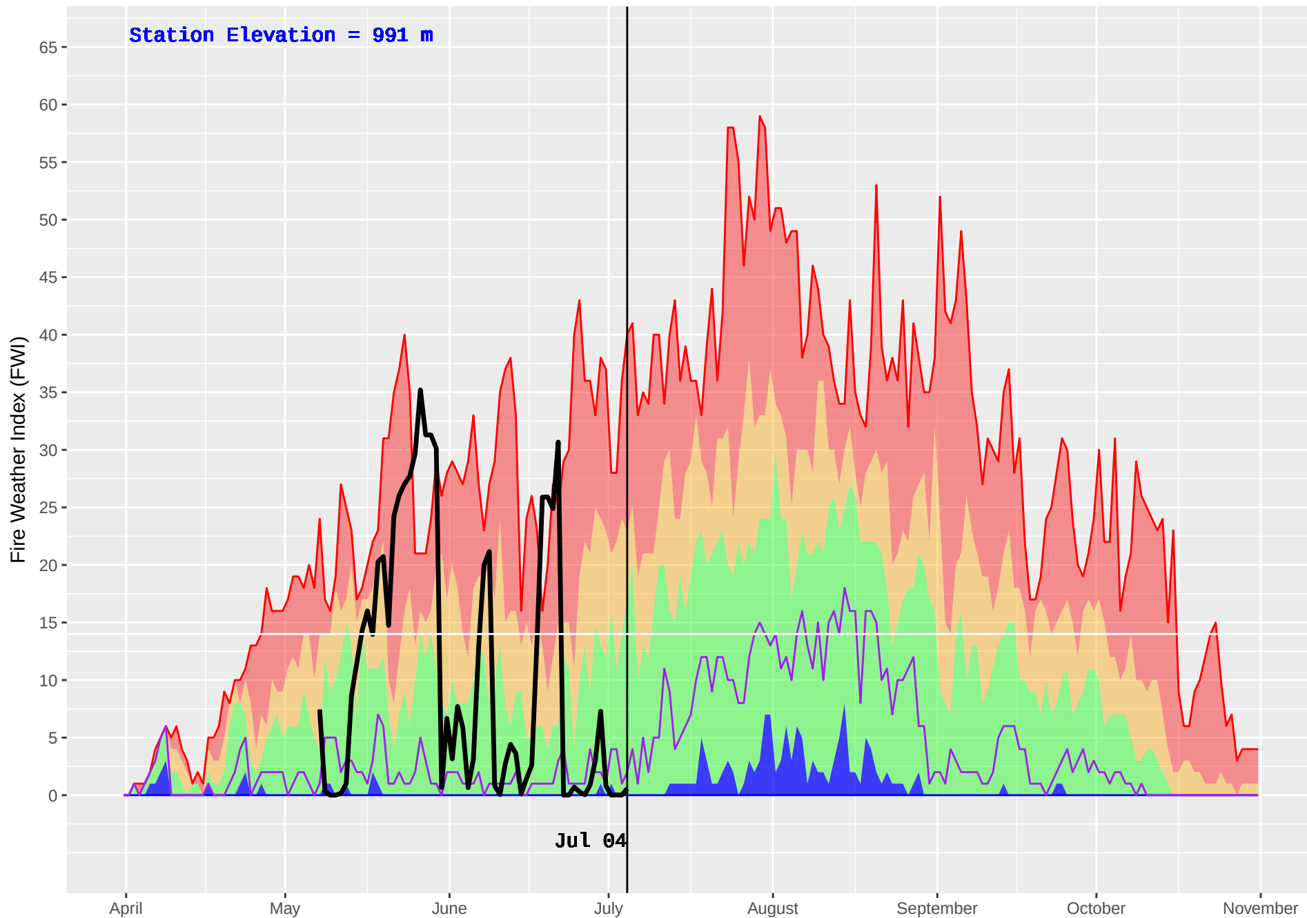
TROUT LAKE (387) : Historical (1987–2016) and Current (2018) Noon Fire Weather Index (FWI)
