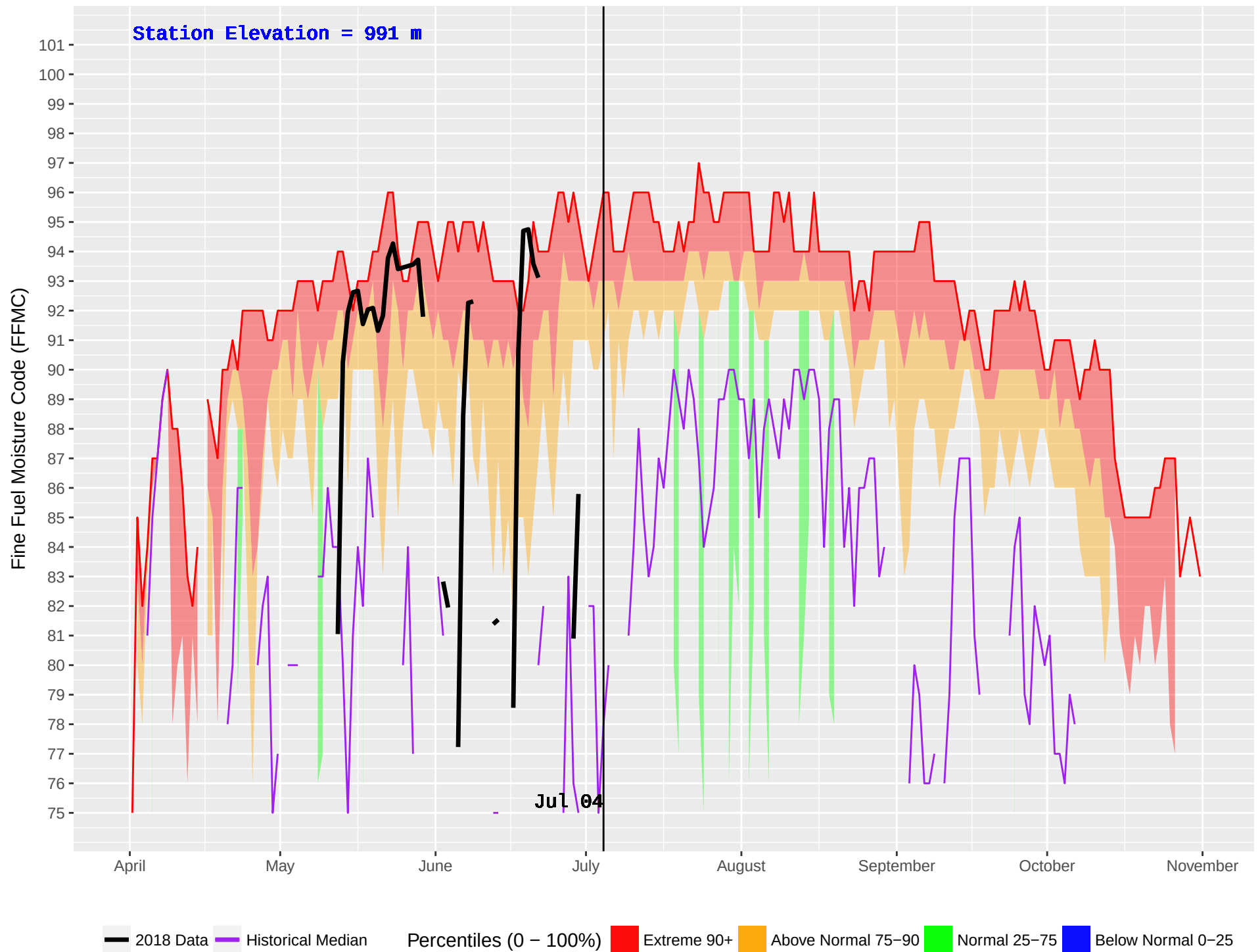
TROUT LAKE (387) : Historical (1987–2016) and Current (2018) Noon Fine Fuel Moisture Code (FFMC)
